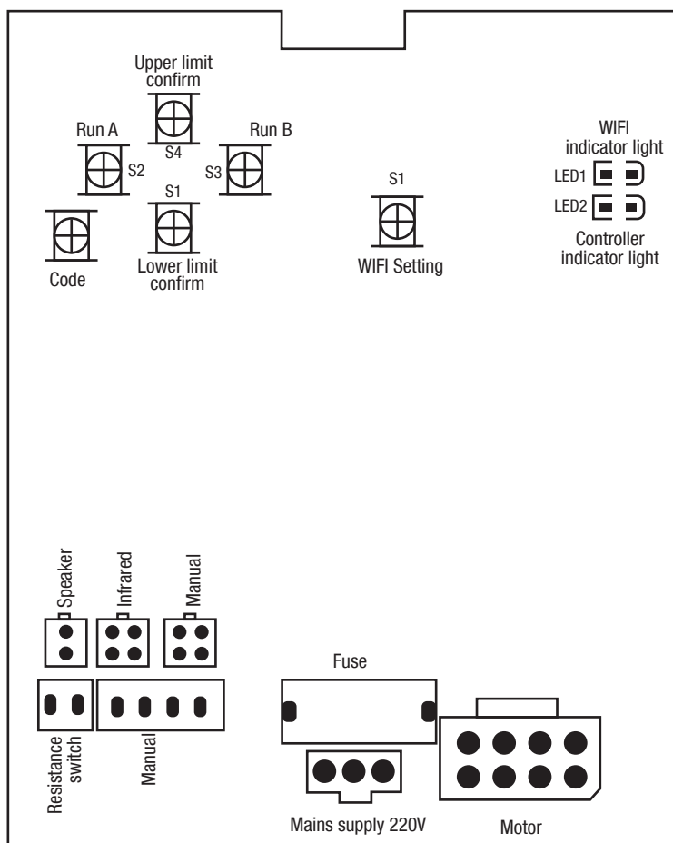
System Connection Debugging Diagram (Fig.1)
